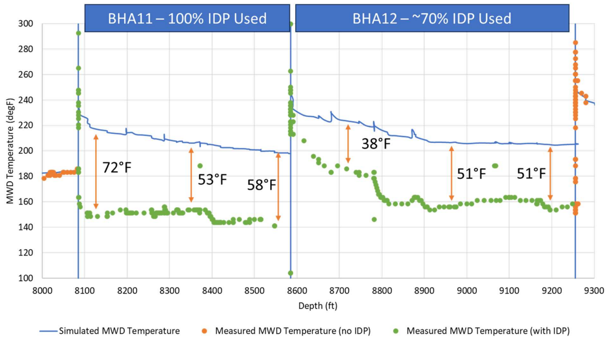
Figure 5: BHA temperature prediction, assuming non-insulated Drill Pipe (zoom into the BHA 11 and 12)
