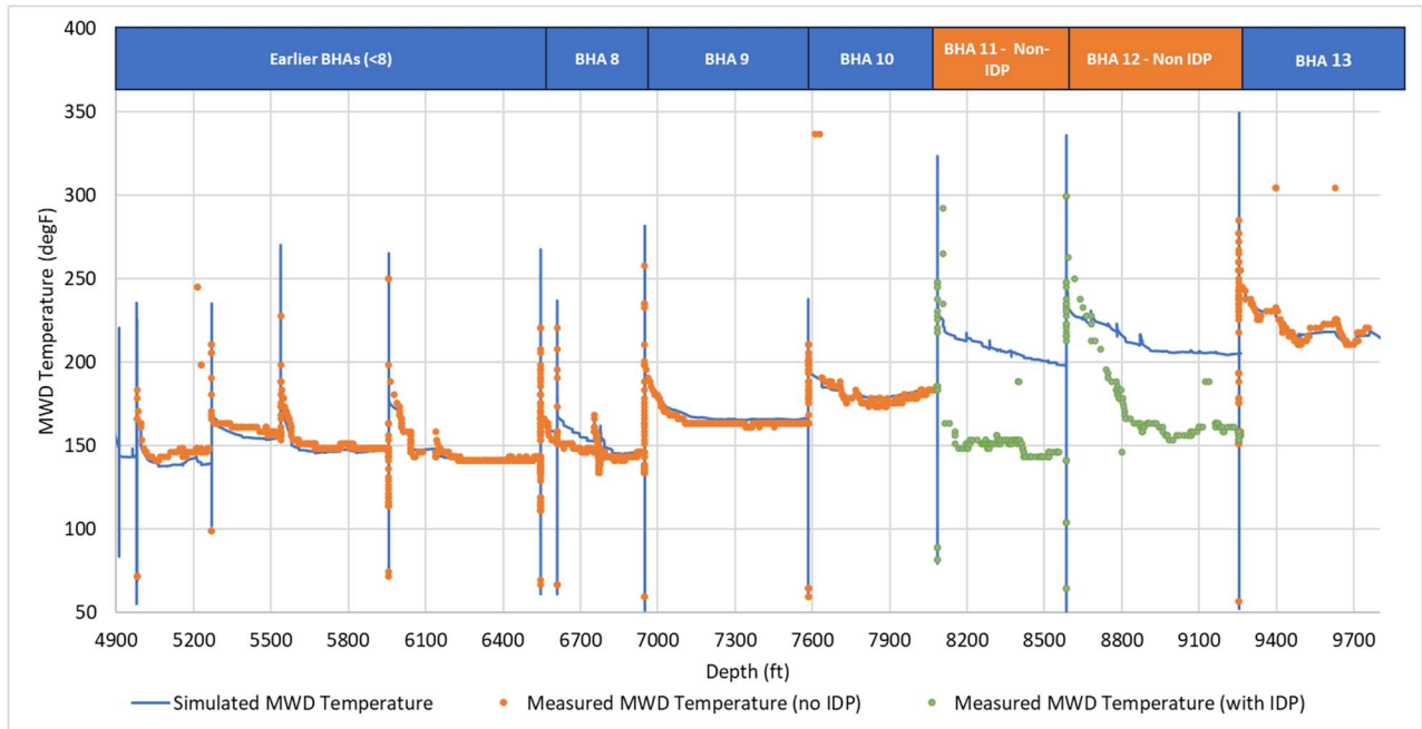
Figure 4: the BHA temperature prediction, assuming non-insulated Drill Pipe
