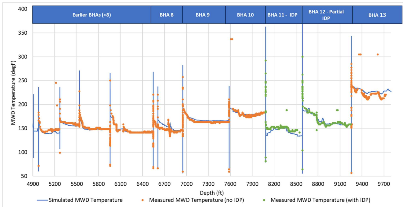
Figure 3: the BHA temperature prediction using Eavor’s Transient Drilling Model
