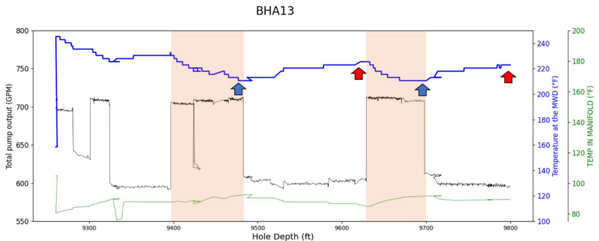
Figure 2: Impact of flow rate on MWD temperature
