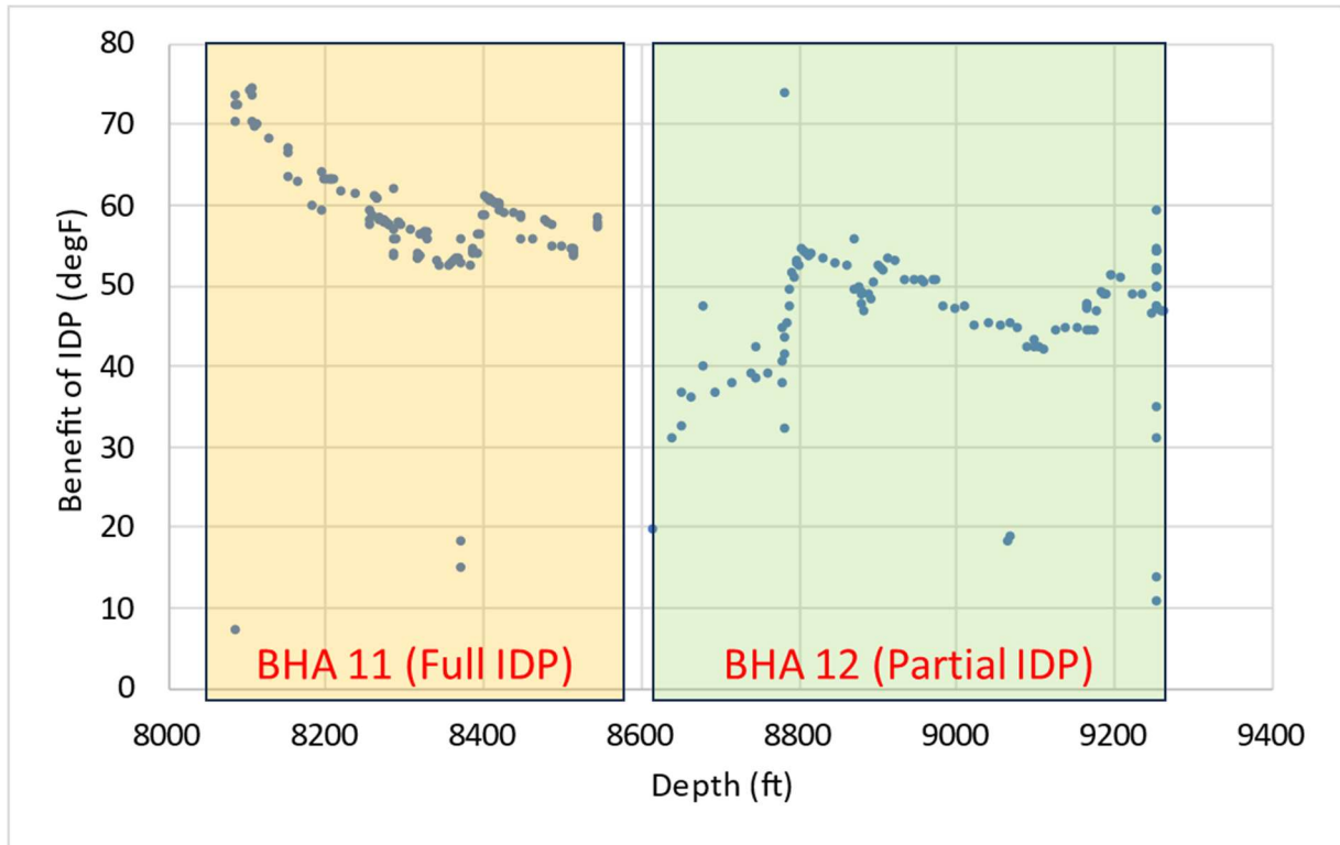
Figure 6: Benefit of the IDP (modelled bottomhole circulating temperature without the IDP minus measured bottomhole circulating temperature with the IDP)
