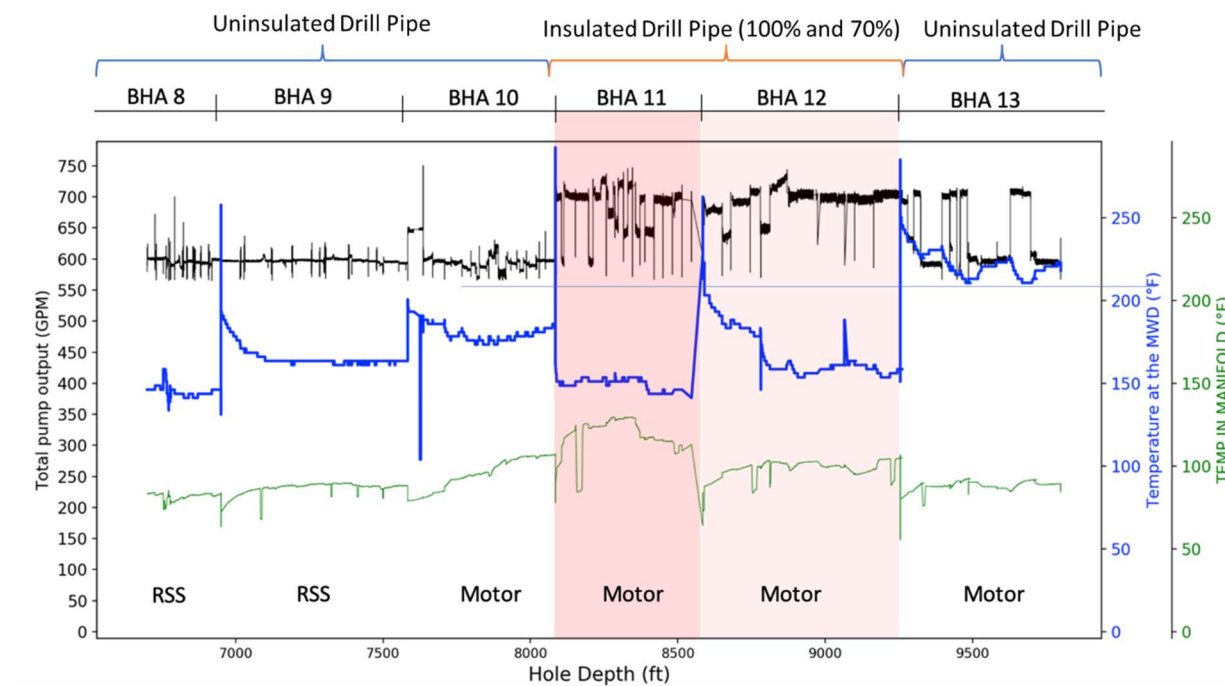
Figure 1: Pump output, Inlet Temperature and MWD Temperature vs Depth
